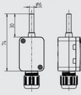
Model TF41 with probe sleeve
