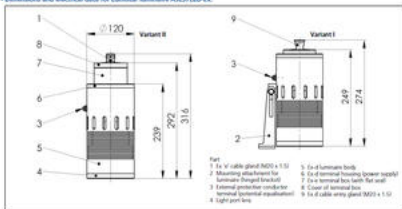
Dimensions and electrical data for Luminaire luminaires ASL57LED-Ex
