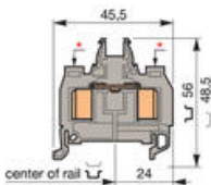
Standard 8 mm plint. Bredd 8 mm.
